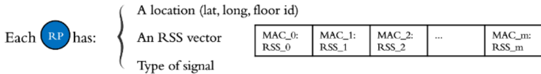
Figure 5.8: The structure of a reference point
