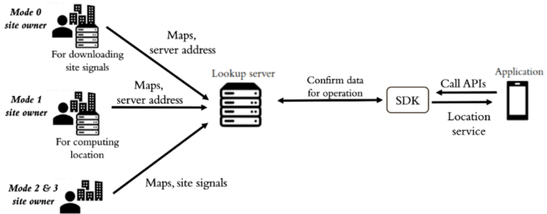
Figure 5.7: A holistic view of communication protocols
